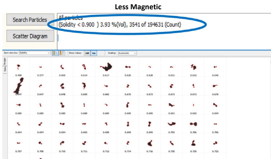
Fig. 5: Sample images from Microtrac SYNC for Less Magnetic sample showing evidence of agglomeration. Selection parameter used was Solidity where a value of "1" indicates smooth surface. Agglomerates such as those shown have much lower values than "1". The Search function indicates that approximately 3% (by volume) of the sample has a solidity of less than 0.9.
