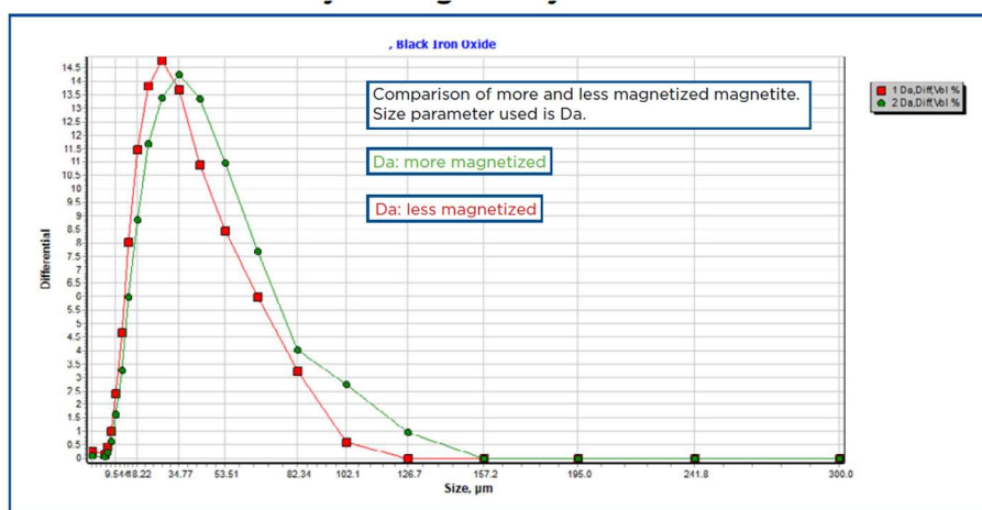
Fig. 4: Graphing capability of FLEX software provided the SYNC image analysis comparison graph. The sensitivity of the measurement is made apparent. Note similarity to diffraction data for the parameter Da.
