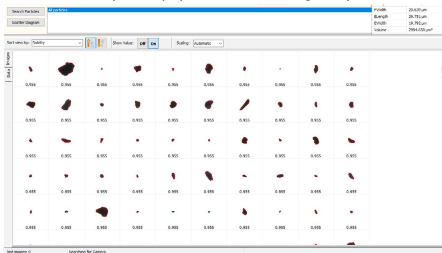
Fig. 7: Sample of images from Microtrac SYNC for Less Magnetic sample showing particles of low agglomeration. Selection parameter used was Solidity where a value of “1” indicates smooth surface. Highest value attained for this sample was 0.99. The Search function indicates that approximately 97% (by volume) of the sample has a solidity of greater than 0.9.
