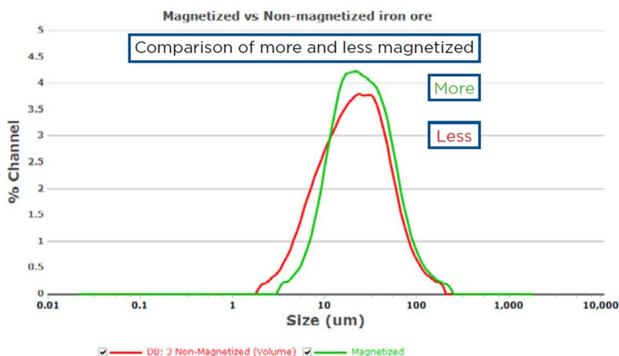
Fig. 2: Graphing capability of FLEX software provided the comparative SYNC diffraction measurement graph. The sensitivity and ability to distinguish small distribution differences of the measurement is made apparent.
