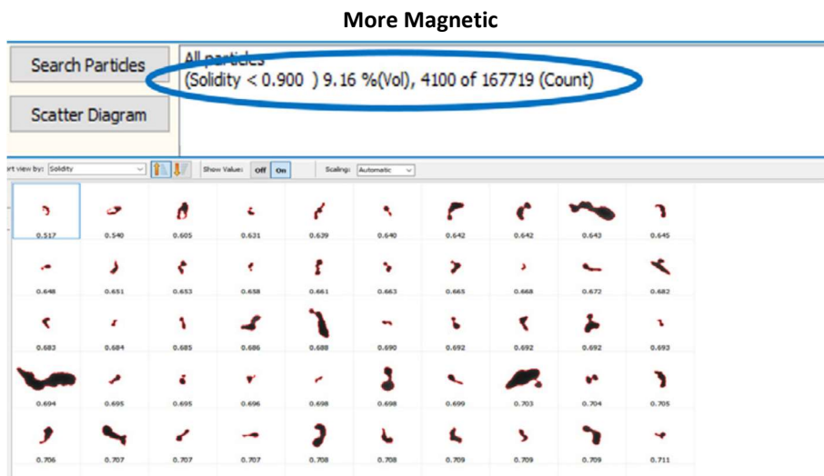
Fig. 6: Sample images from Microtrac SYNC for More Magnetic sample showing evidence of agglomeration. Selection parameter used was Solidity where a value of "1" indicates smooth surface. Agglomerates such as those shown have much lower values. The percent less than a Solidity is shown by the Search function to be approximately 9%. This indicates greater magnetic agglomeration than the previous sample.
